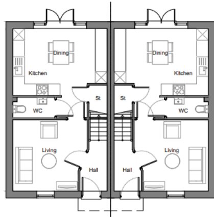
Ground Floor Plan 2840 @ 79.6m 2 / 8571ft 2
