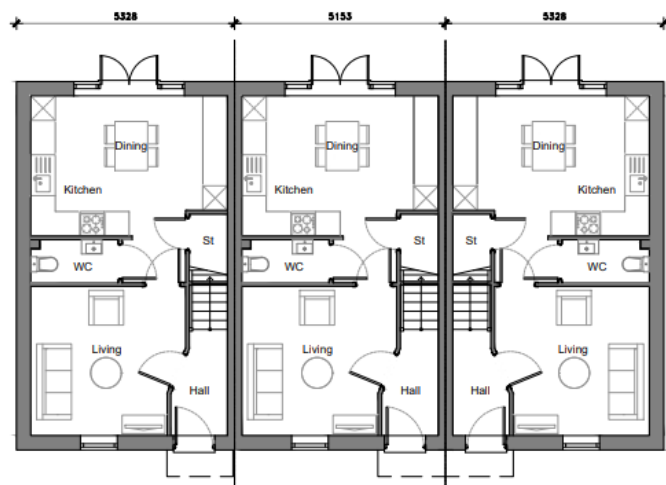
Ground Floor Plan 284P @ 79.6m 2 / 8578 ft
